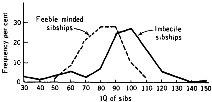
FIGURE 3. Frequency distributions of the IQs of sibs of feebleminded and imbeciles of the IQ range 30-68. (Roberts, 1952.)
